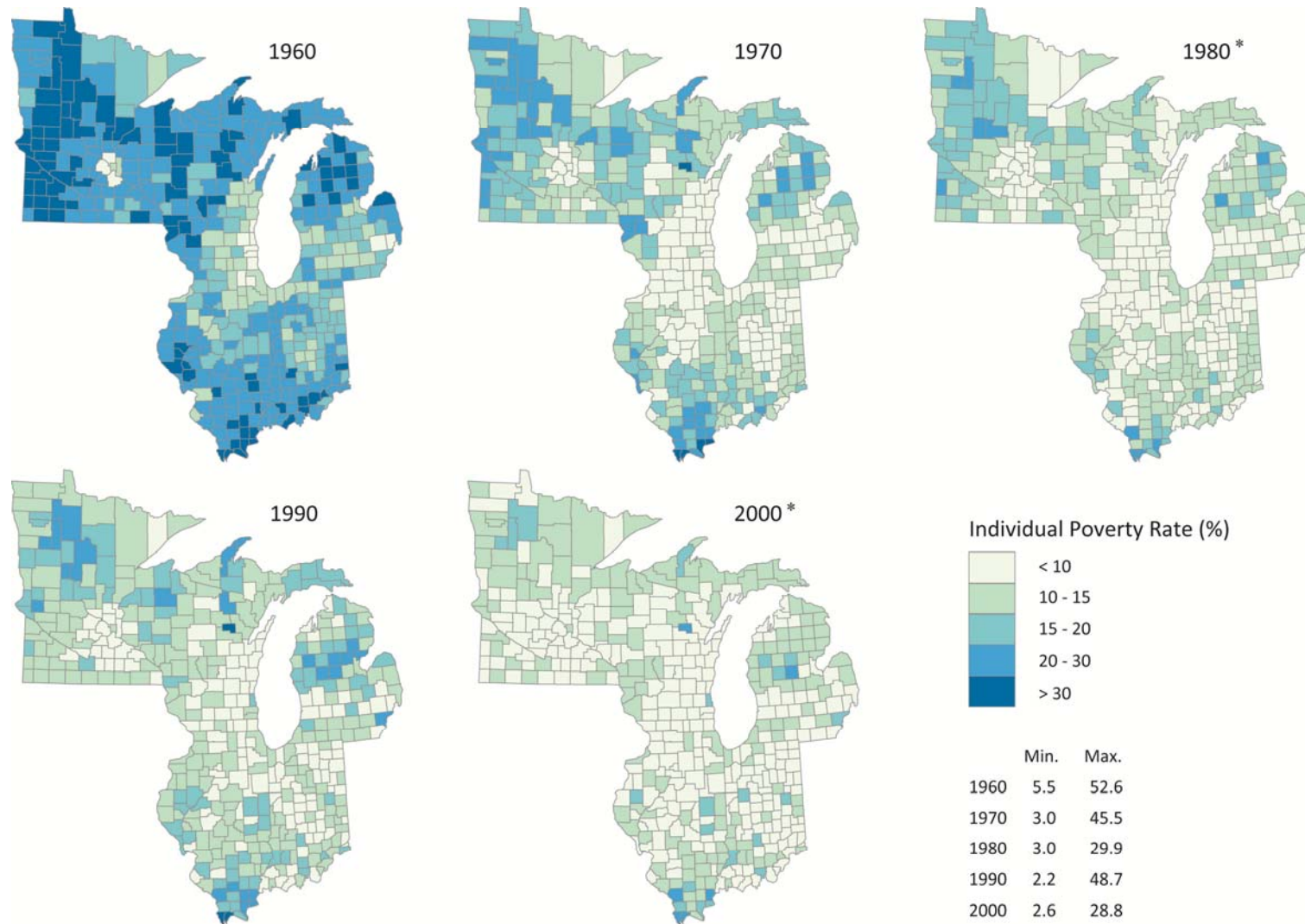
Figure 1. Decade-specific county poverty rates with minimum and maximum values. Upper Midwest counties, 1960-2000.
