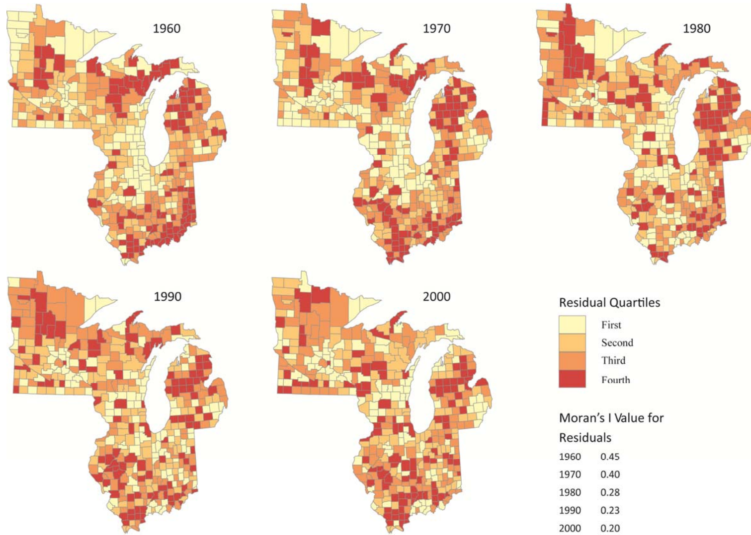
Figure 2. Spatial distribution of decade-specific residuals from standard linear regression analysis (OLS) of county poverty with Moran's I statistics for spatial autocorrelation. Upper Midwest counties, 1960-2000.
